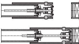
Telescopic element
