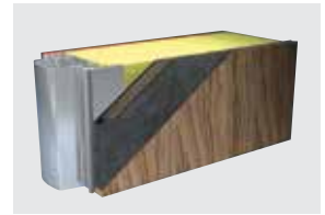
Element design I Construction Page 20–21
